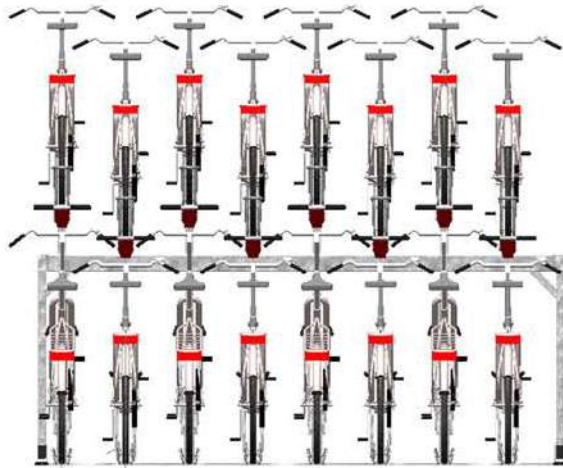
Single sided staggered layout
